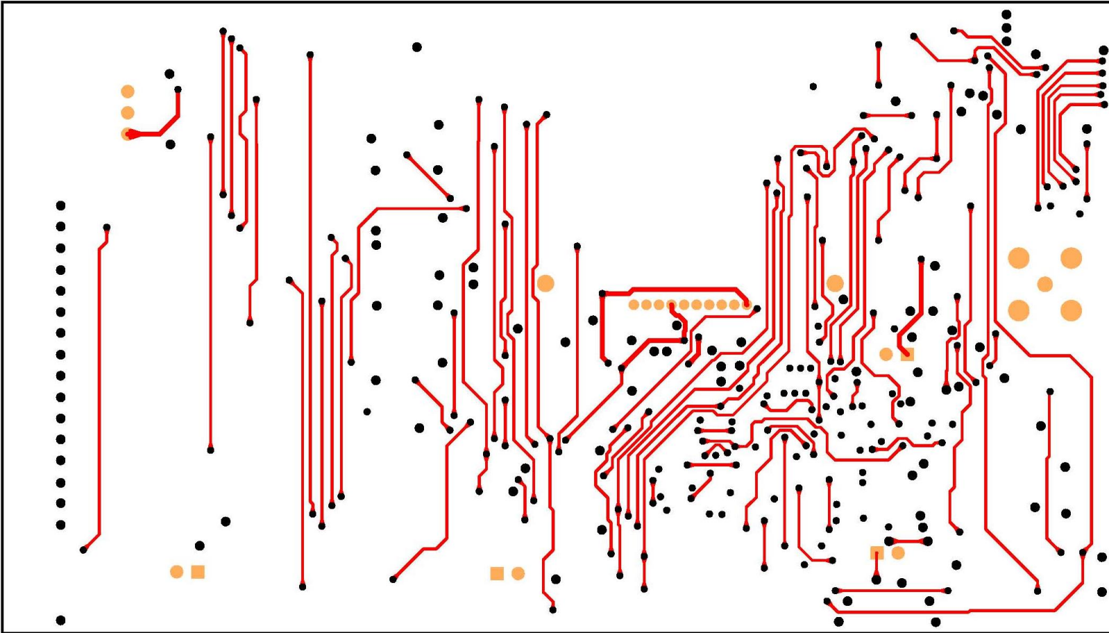
Figure 12: Bottom Layer Layout
