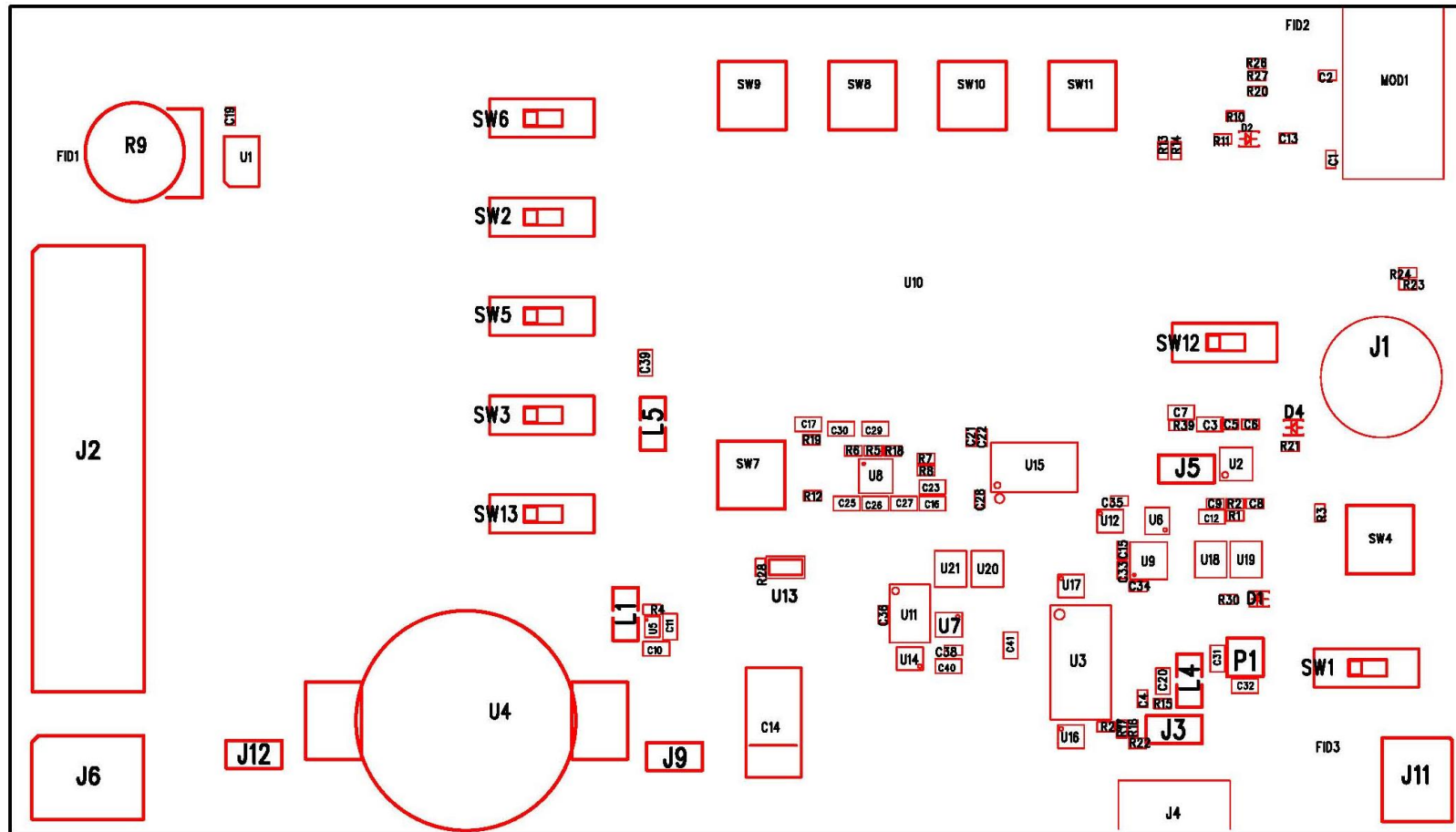
Figure 8: BLE113 Development Board Assembly Drawing
