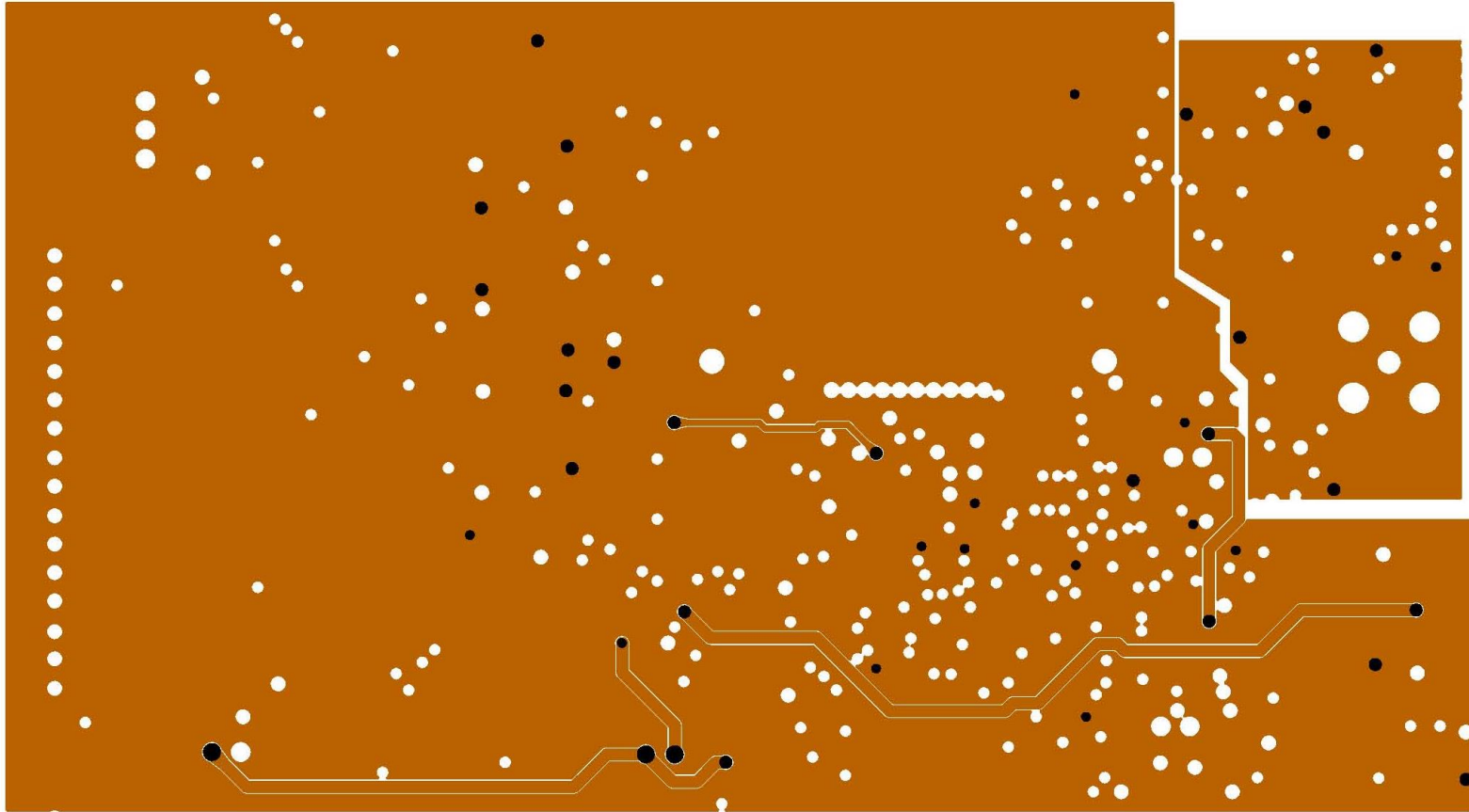
Figure 11: 3rd Layer Layout
