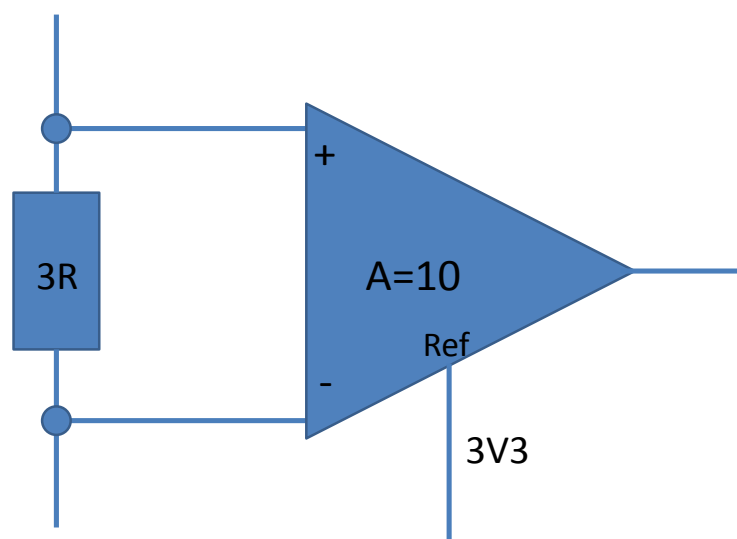
Figure 13: TX current measurement amplifier
