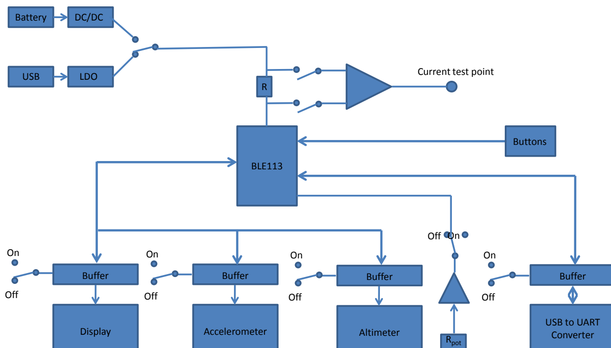
Figure 1: Block diagram of BLE113 evaluation board
