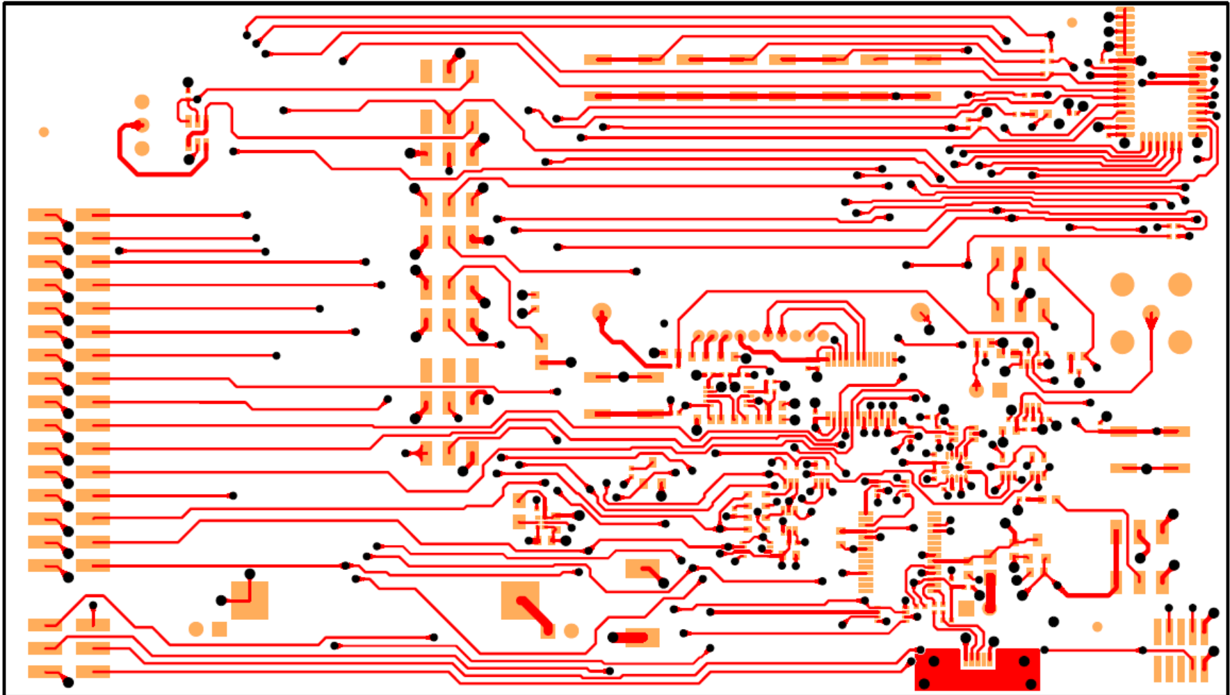
Figure 9: Top Layer Layout
